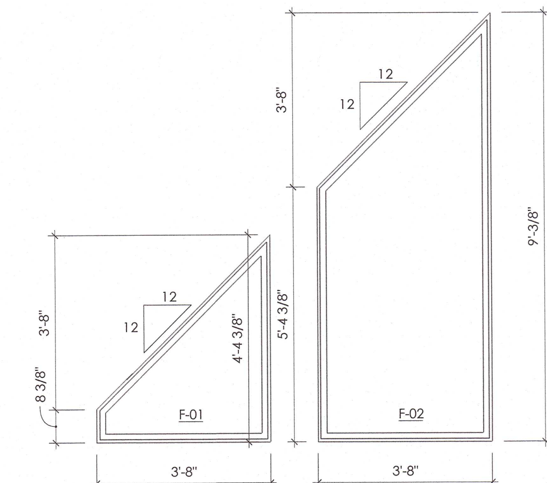
3/14 Fixed Glass Detail SCALE: 1/2" = 1'-0"
